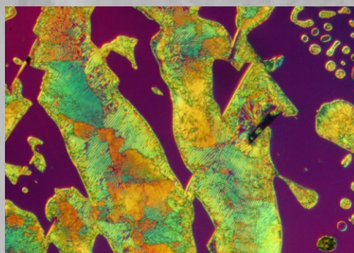
White iron, etch 2% Nital, 1000X (DIC)
